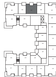
LEVEL 4
