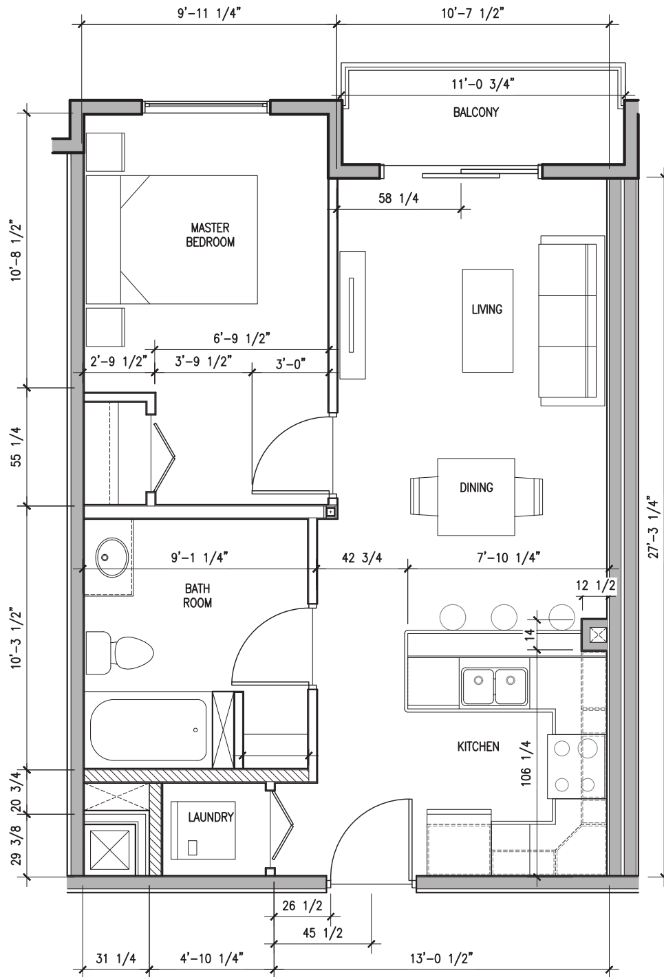
SUITE TYPE A1c
